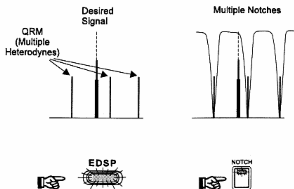
EDSP Auto Multiple Notch Action
