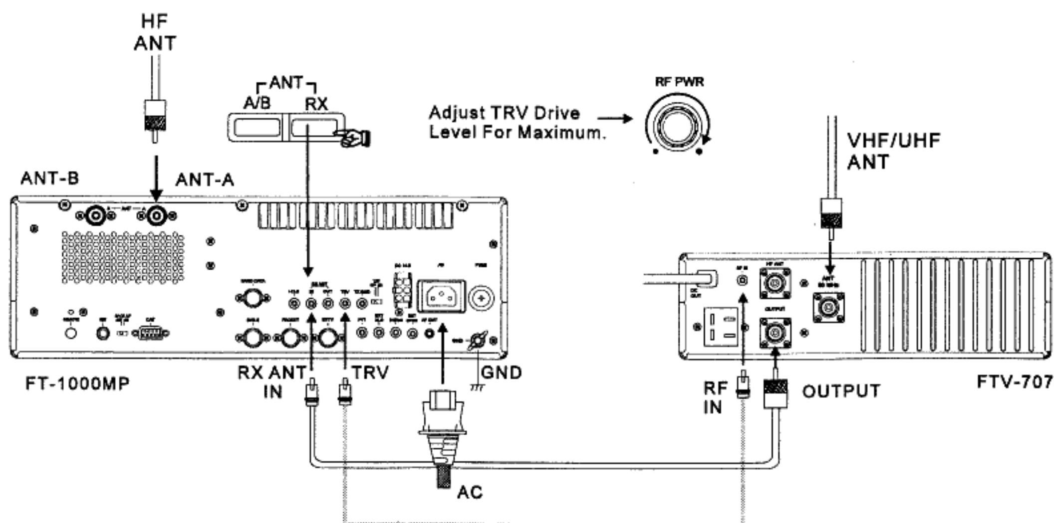
Example of Transverter Station Interconnections
