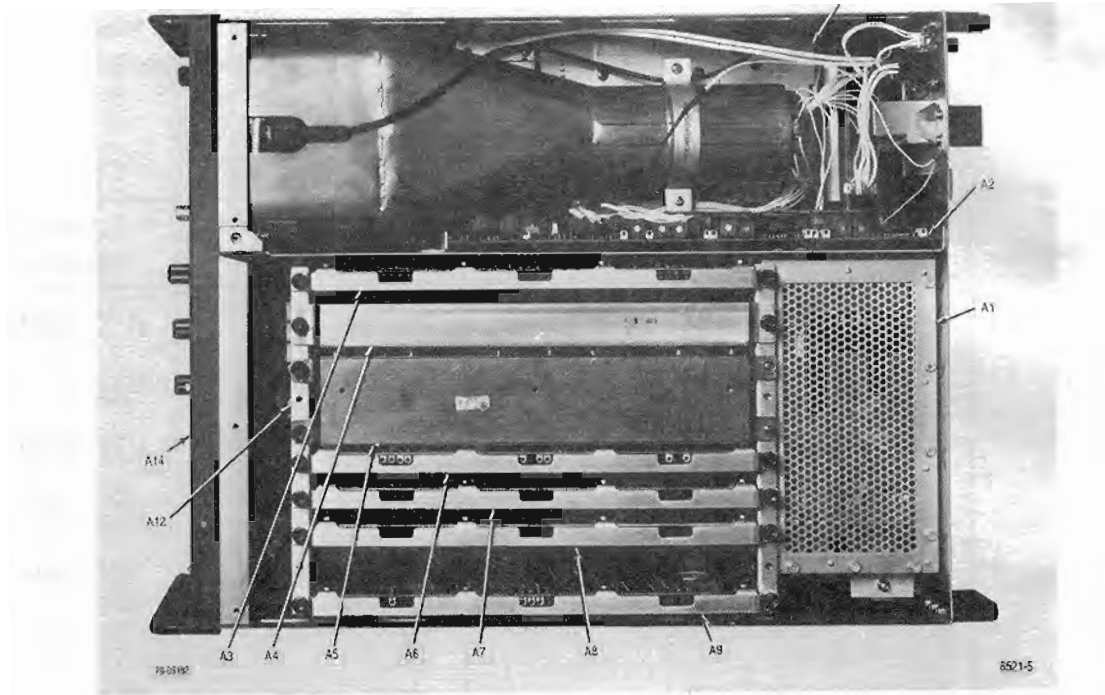
Figure 5-1. Communication System Analyzer, Top View Cover Removed
