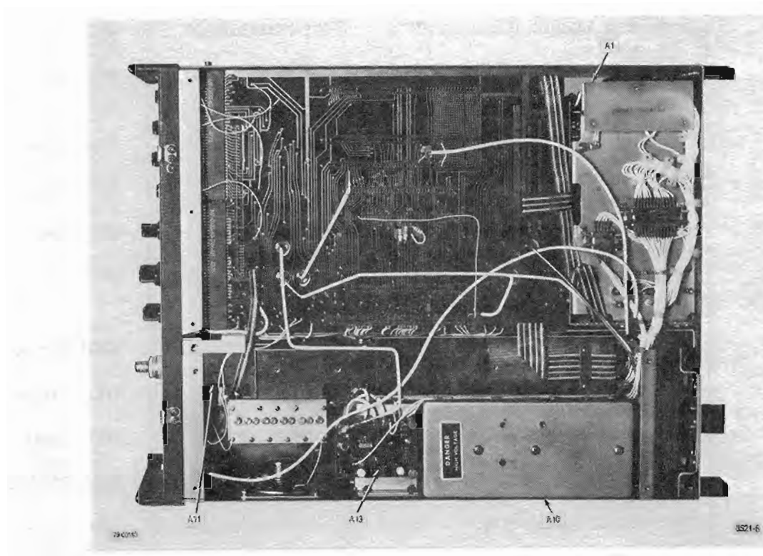
Figure 5-2. Communication System Analyzer, Bottom View Cover Removed
