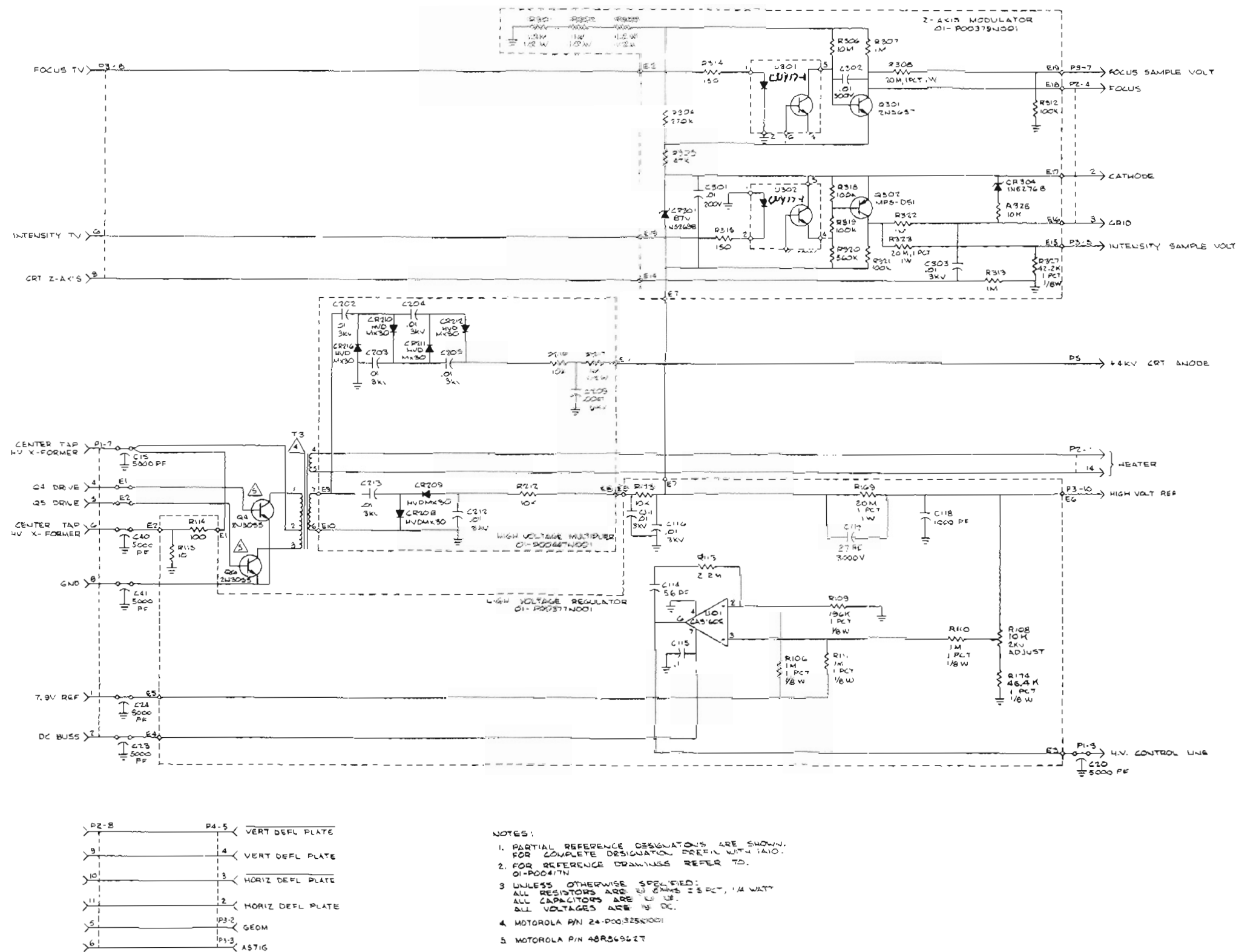
Figure 16-2. High Voltage Power Supply A10 Schematic Diagram (RTP-1001A)
