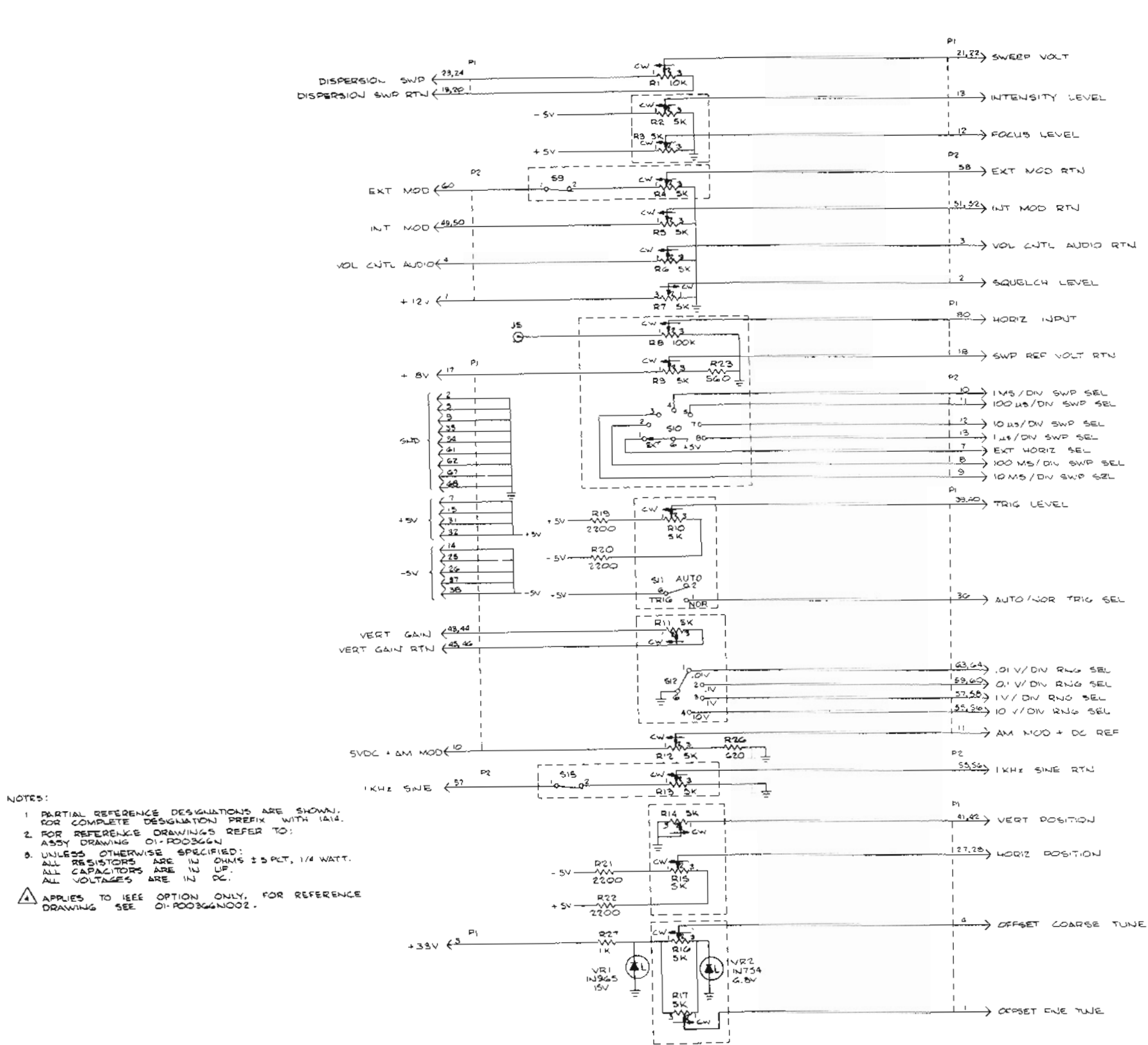
Figure 20-1. Front Panel A14 Schematic Diagram (Sheet 1 of 3) (01-80304A42)
